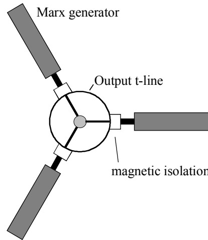
Figure 5. Generator interconnection with output transmission line
