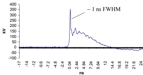
Figure 4. A typical output pulse from the APELC Marx generator.
