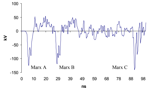
Figure 8. Output waveform of the Gatling system measured with a capacitive probe.
