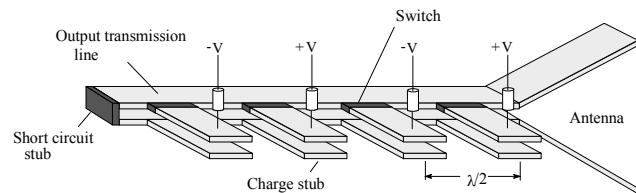
Figure 1. The Injection Wave Generator.
