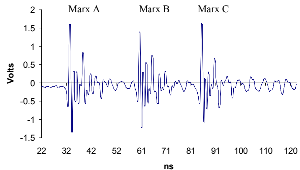
Figure 9. Radiative results from the Gatling system.
