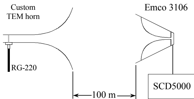
Figure 7. Radiation measurements setup.
