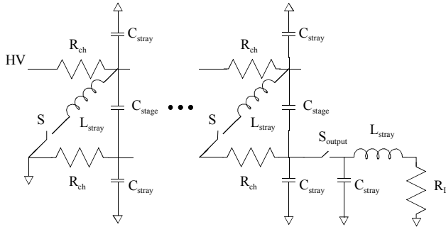
Figure 3. The Wave-Erection Marx Generator.
