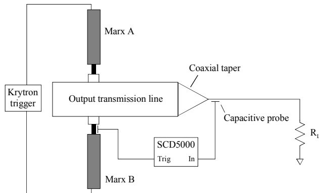
Figure 6. Experimental arrangement.
