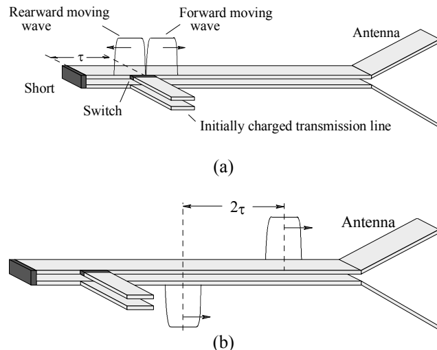
Figure 2. Propagation and spatial dependence of the injected waves, (a) launched waves, (b) resulting propagation.
