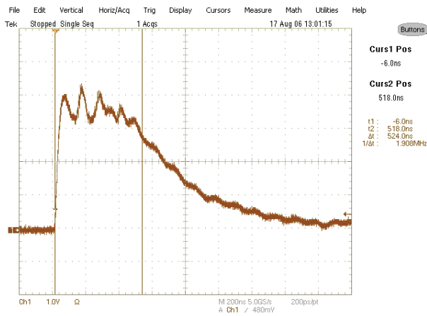
Figure 9. Sample Output Waveform with 1.3 \mu\text{H} Isolation Inductors
