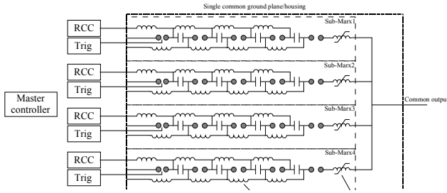
Figure 2. Basic Schematic for the Sequentially Switched Marx Generator System
