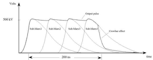
Figure 1. Illustration of Sequentially Delivered High Voltage Pulses to a Common Load
