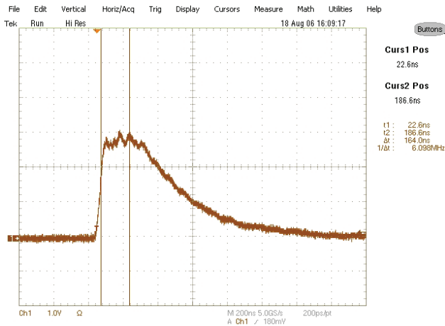
Figure 10. Sample Output Waveform with 2.3 \mu\text{H} Isolation Inductors
