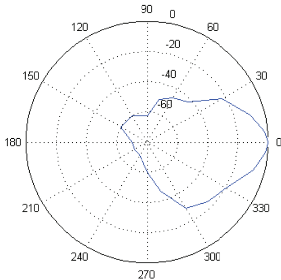
Figure 7. Measured antenna pattern for 6-ft Radiating Dish. The pattern given is a ratio of the measured field at each angular location (in degrees) to the maximum measured field in decibels.
