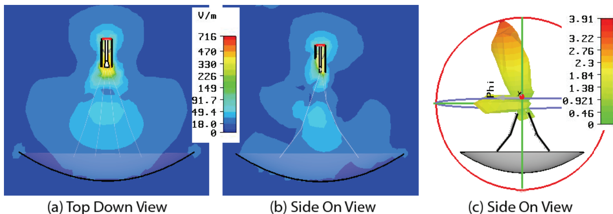
Figure 4. (a) A top down view of a near field cross-section of the IRA system excluding the Marx generator. (b) A side on view of a near field cross-section of the IRA system excluding the Marx generator. (c) Side on view of the far field gain from the IRA system.
