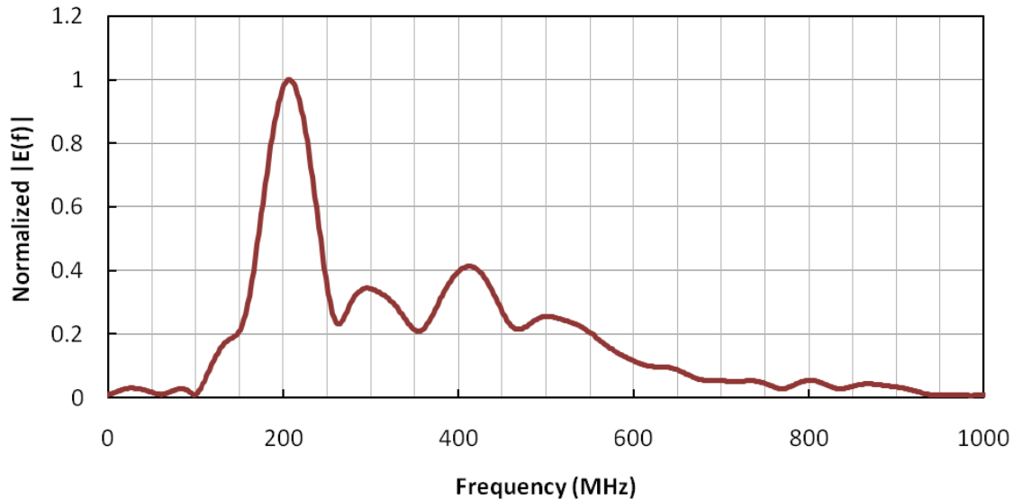
Figure 6. Spectral content of the radiated signal shown in Figure 5.
