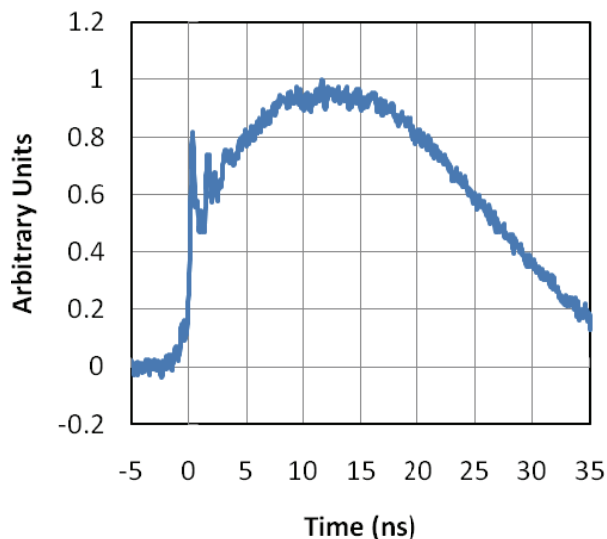
Figure 2. Example Marx generator waveform from testing with a cable load.
