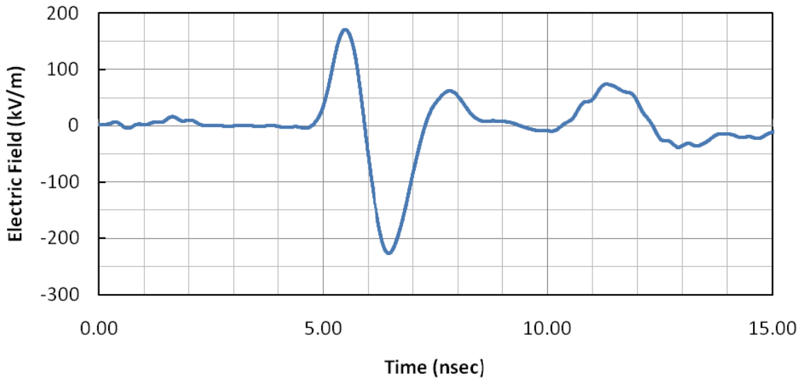
Figure 5. Experimentally measured radiated electric field normalized to a range of 1 meter.
