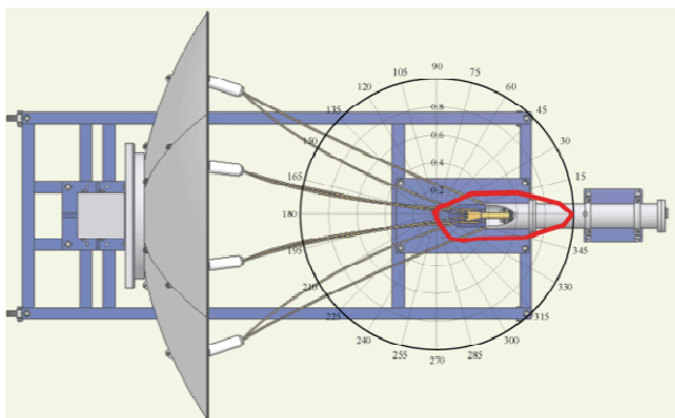
Figure 8. The orientation of the field pattern with respect to the system.
