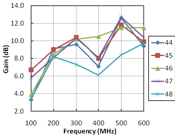
Figure 3. The dependence of relative position of Marx to parabolic reflector on system gain at several frequencies of interest. The legend indicates the relative distance between the source and the parabolic dish.
