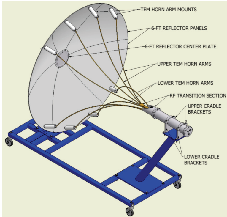
Figure 1. (a) Major components of the APELC 6-ft IRA. (b) Major components comprising the RF transition section, the parabolic reflector, and the Marx generator mounting hardware.
